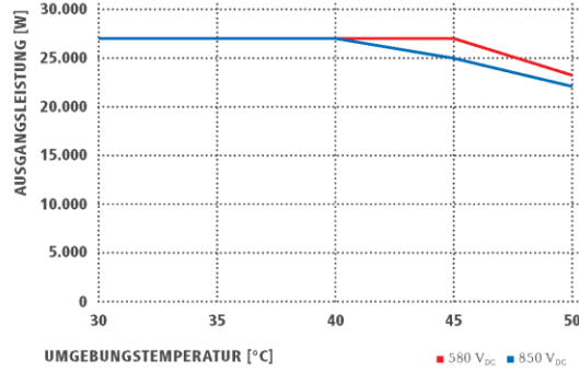
TEMPERATURDERATING FRONIUS ECO 27.0-3-S
